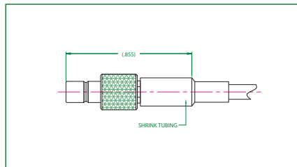
Straight Jack NM 3500 - 1630 - 5400
